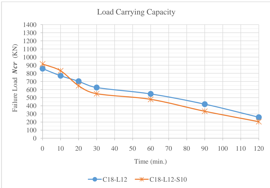
Figure13: lost of confinement effect for modelC18-L12-S10
