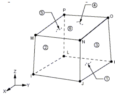
Figure 3: Solid180 Geometry
