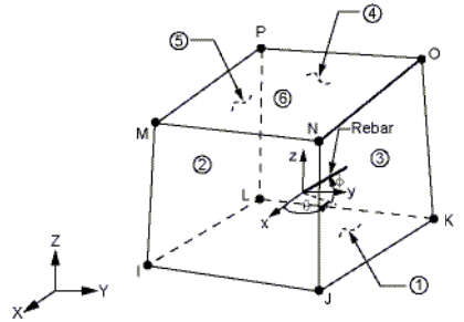
Figure 1: SOLID65 Geometry
