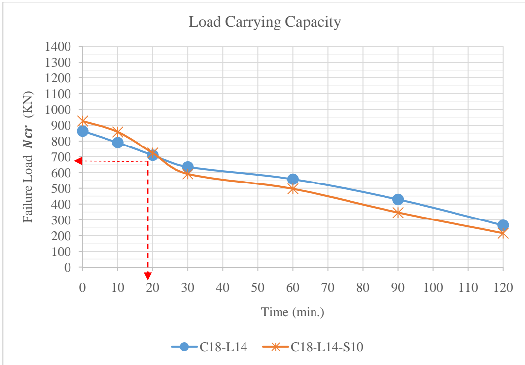
Figure16: lost of confinement effect for modelC18-L14-S10
