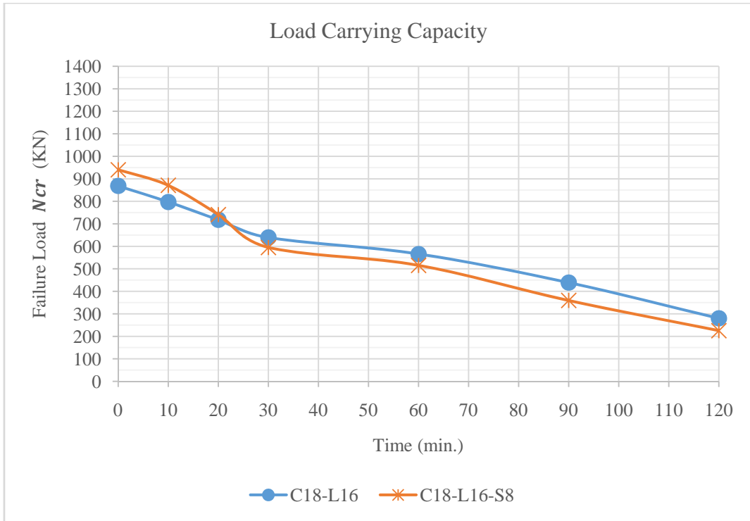
Figure18: lost of confinement effect for modelC18-L16-S8
