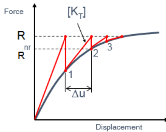
Figure 7: Newton-Raphson method
