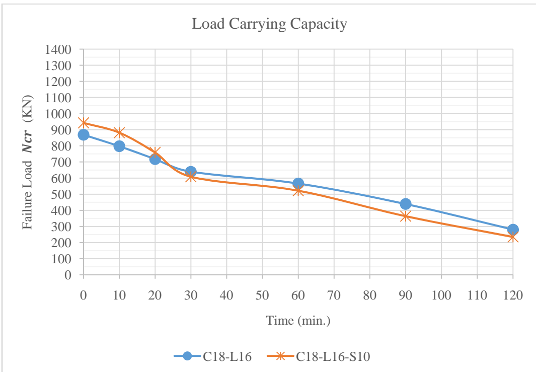
Figure19: lost of confinement effect for modelC18-L16-S10
