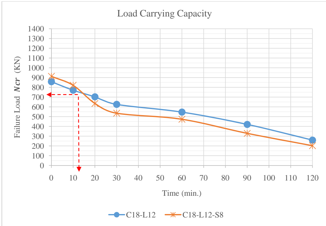
Figure12: lost of confinement effect for modelC18-L12-S8
