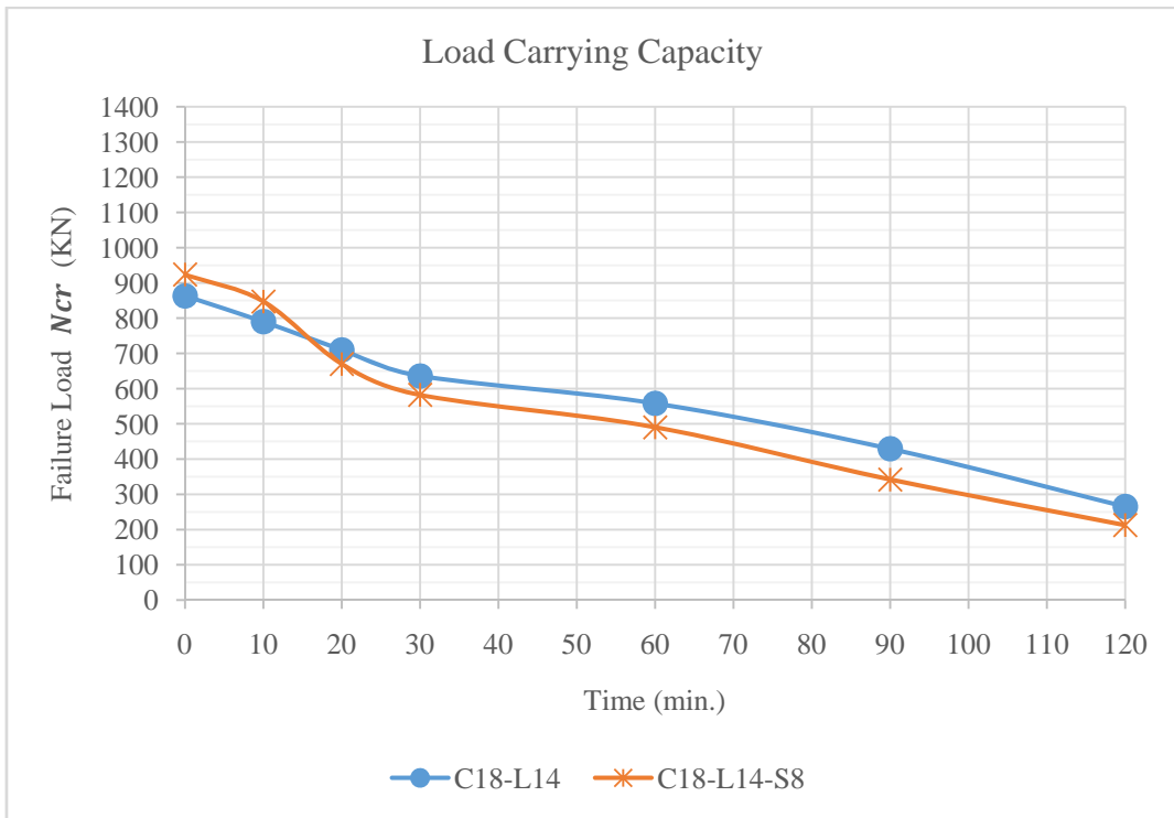
Figure15: lost of confinement effect for modelC18-L14-S8
