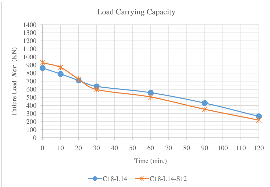
Figure17: lost of confinement effect for modelC18-L14-S12
