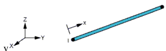
Figure 2: LINK180 Geometry
