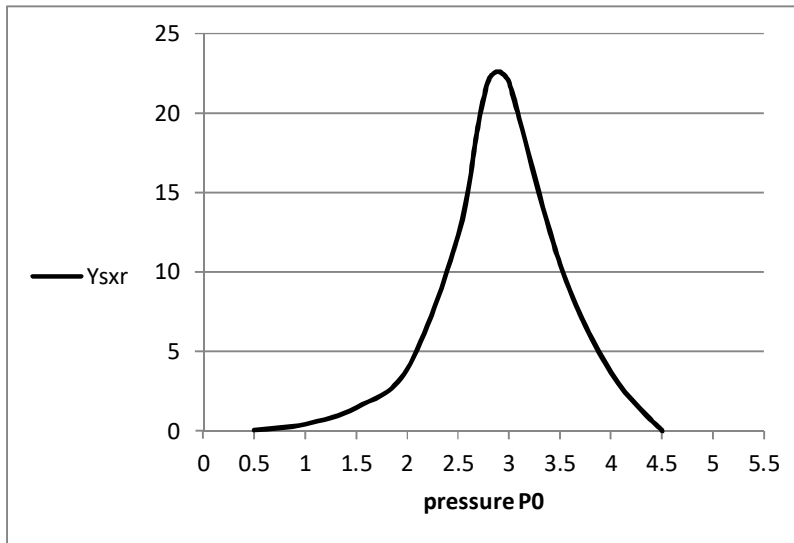
FIG. 1. Soft x-ray yield as a function of pressure.
