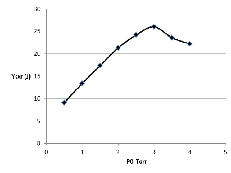
FIG. 5. Soft x-ray yield as a function of pressure, anode length and inner radius.
