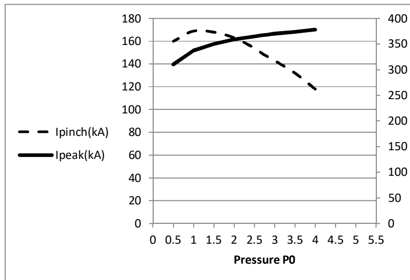
FIG. 3. Variation of I_{pinch} and I_{peak} versus pressure.
