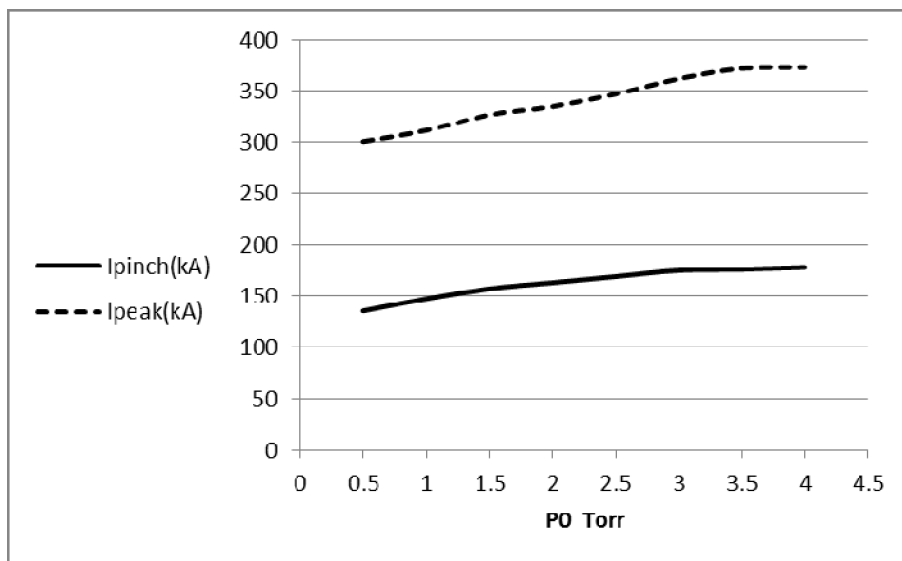
FIG. 6. Effect on total current ( I_{peak} ) and pinch current ( I_{pinch} ) as P_0 is increased from 0.5 to 4 Torr.
