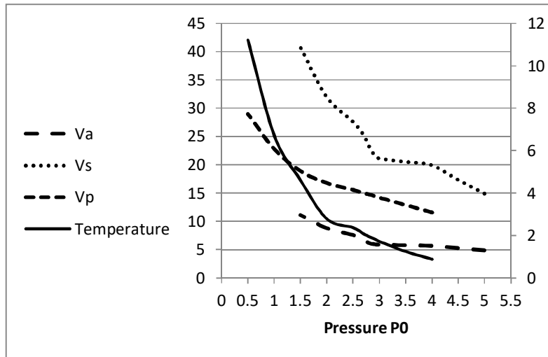
FIG. 2. Speeds and plasma temperature as functions of pressure.
