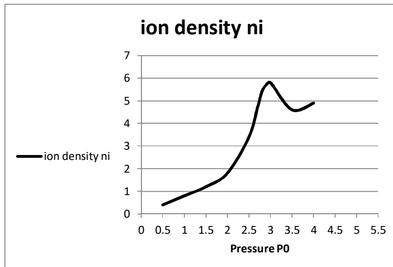
FIG. 4. Variation of ion density versus pressure.
